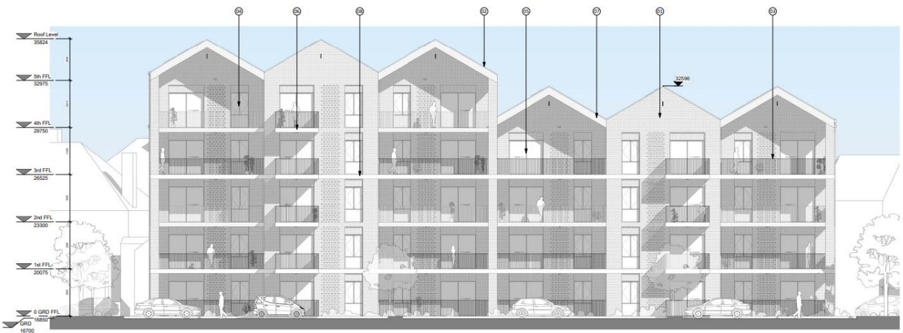
2 2002 - South Elevation (Block A) 1:100
